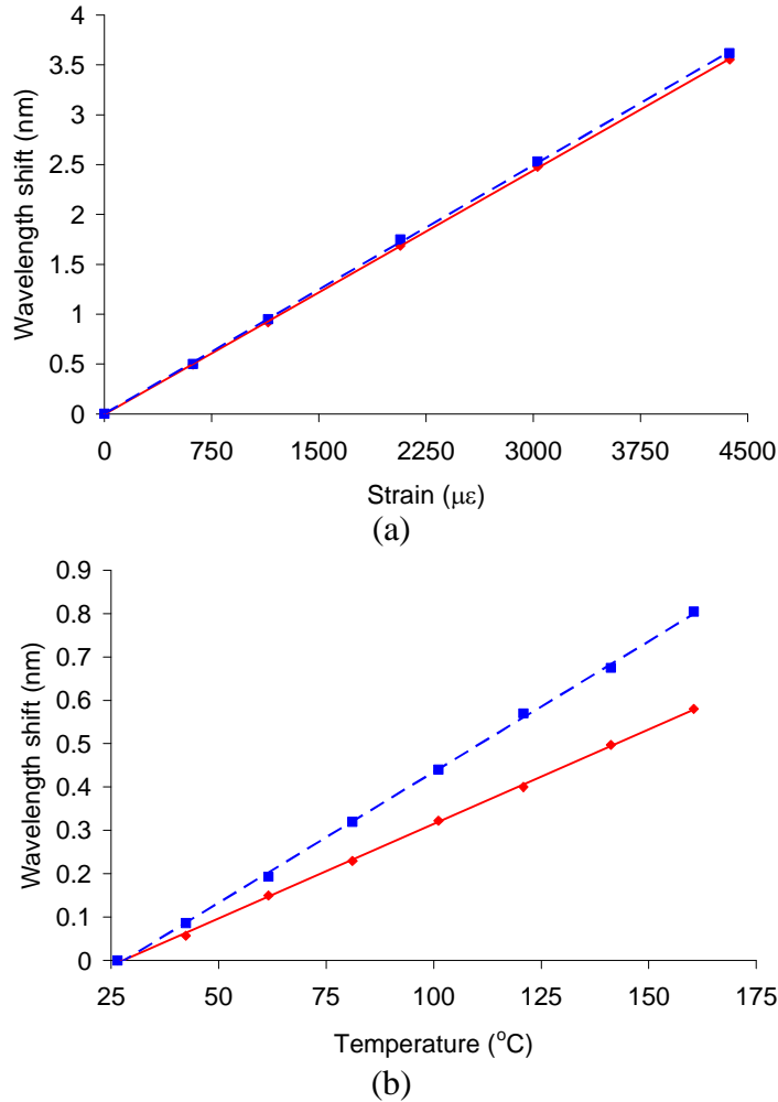
Figure 3 (a) strain and (b) temperature sensitivity of the resonance features of a TFBRG with tilt angle 1.5^{\circ} , fabricated in hydrogen loaded boron-germanium co-doped optical fibre of cut off wavelength 1213 nm. \blacklozenge (red): core-core (Bragg) mode resonance and \blacksquare (blue): core-cladding mode resonance. The lines are best fits to data points.
